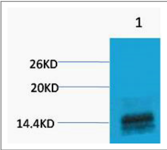
Western blot analysis of 1) Raw264.7, diluted at 1:1000. Secondary antibody (catalog#:RS0002) was diluted at 1:20000 cells nucleus extracted by Minute TM Cytoplasmic and Nuclear Fractionation kit (SC-003,Inventbiotech,MN,USA).
