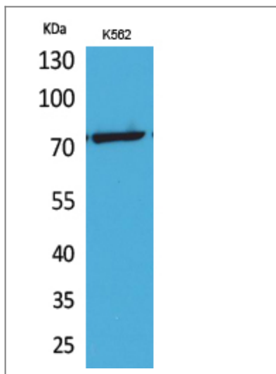
Western Blot analysis of K562 cells using Acetyl-p73 (K321) Polyclonal Antibody. Secondary antibody(catalog#:RS0002) was diluted at 1:20000
